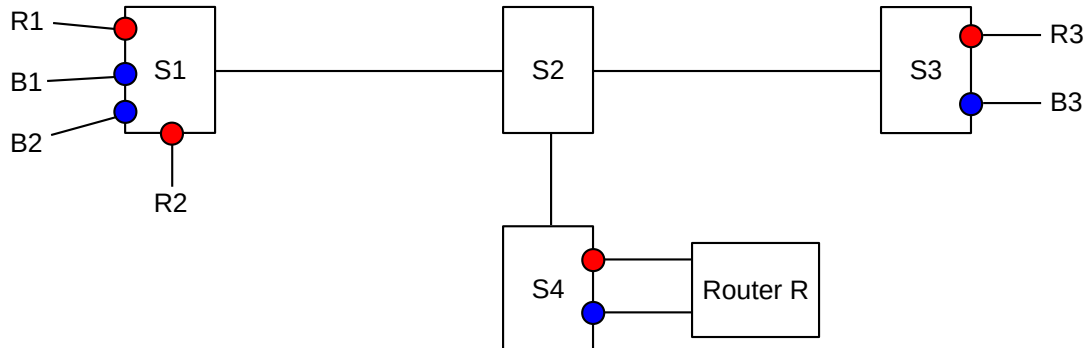
One network of switches S1-S4 divided into two VLANs, red and blue
